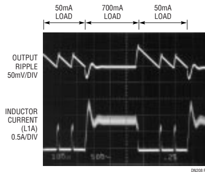
Figure 7. Load Step Response (50mA to 700mA)
