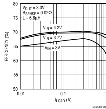
Figure 6. Efficiency vs Output Load Current
