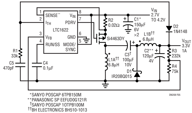
Figure 5. Zeta Converter (3.3V, 1A)
