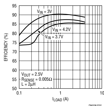
Figure 2. Efficiency vs Output Load Current
