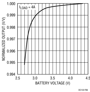
Figure 3. Drop-out Characteristic of Figure 1
