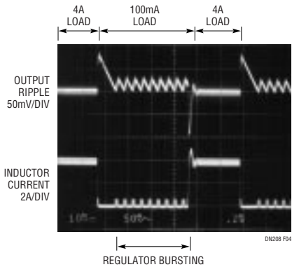
Figure 4. Load Step Response (0.1A to 4A)
